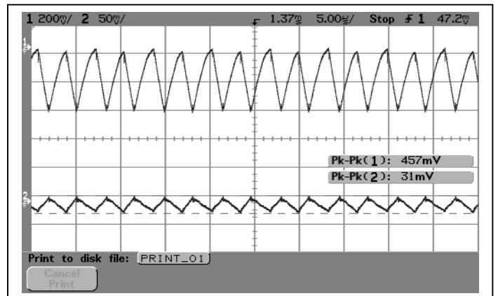
Output voltage noise/ripple (bottom) and input voltage noise/ripple (top) with 2A load current and 16V input voltage. The measurement bandwidth is 20MHz.
