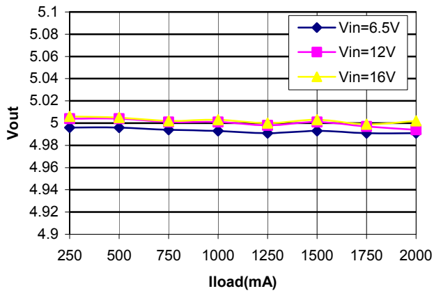
Line and Load Regulation
