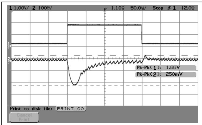
Output voltage transient response (bottom) with load current (top). The load current steps from 200mA to 1.8A to 200mA. Vin = 6.5V, measurement bandwidth is 20MHz.
